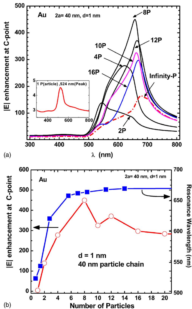
FIG. 2. (Color online) (a) |E| enhancement at hot spot C in a gold nanoparticles chain with different numbers of same sized particles, as a function of wavelengths. (b) presents the corresponding peak enhancement value and resonance wavelength extracted from (a).
