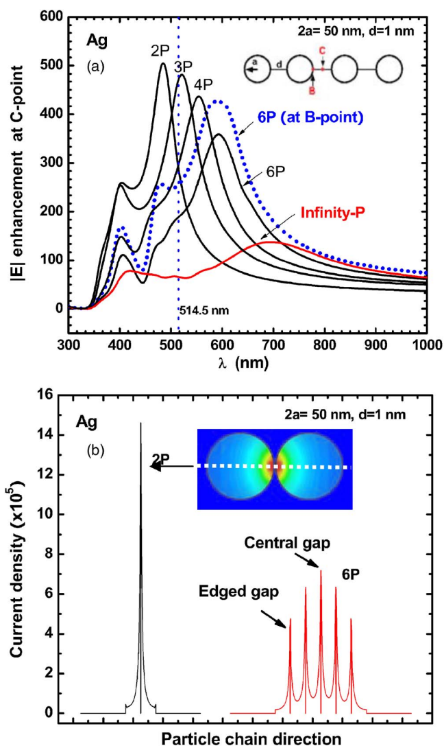
FIG. 1. (Color online) (a) |E| enhancement at the middle of the central gap (hot spot C as in inset) in a silver nanoparticle chain with different numbers N of 50 nm particles, as a function of wavelengths. Also shown is the maximum enhancement on the particle surface for N=6 particle chain. (b) Corresponding current density distribution across the particle chain centers for N=2 and N=6 particle chains.
